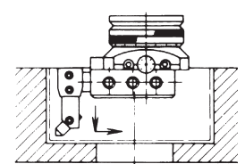
Boring and tacing with short boringbar holder and a boringbar
