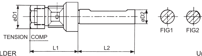
HOLDER
