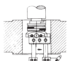
Recessing
