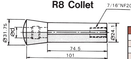
R8 Collet
